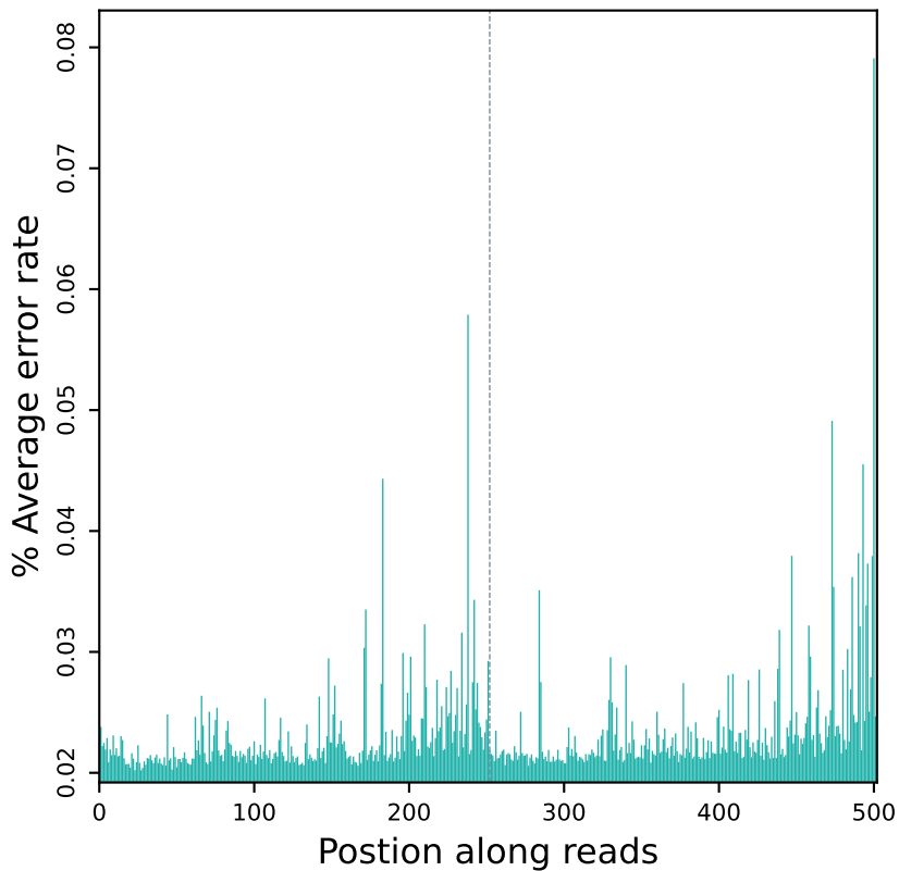
Error rate distribution along reads (R10125)
